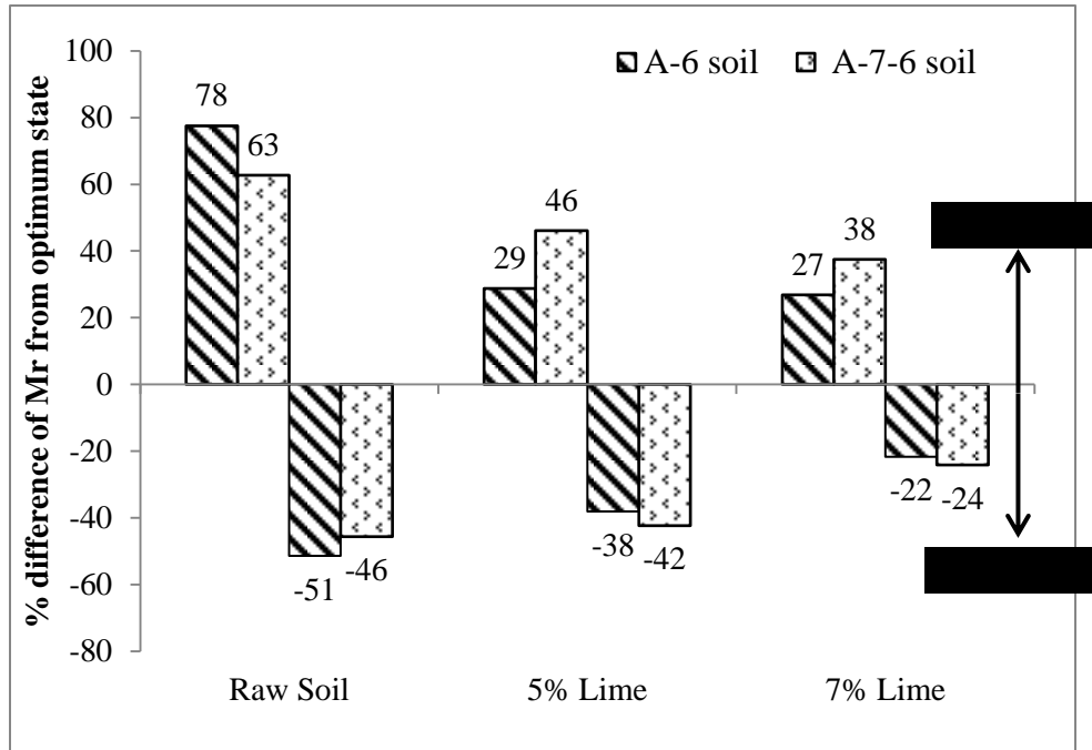
Figure 4.13 Percent Difference from Optimum Moisture in Resilient Modulus Results
