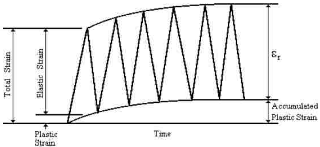
(b) Strains under repeated load
